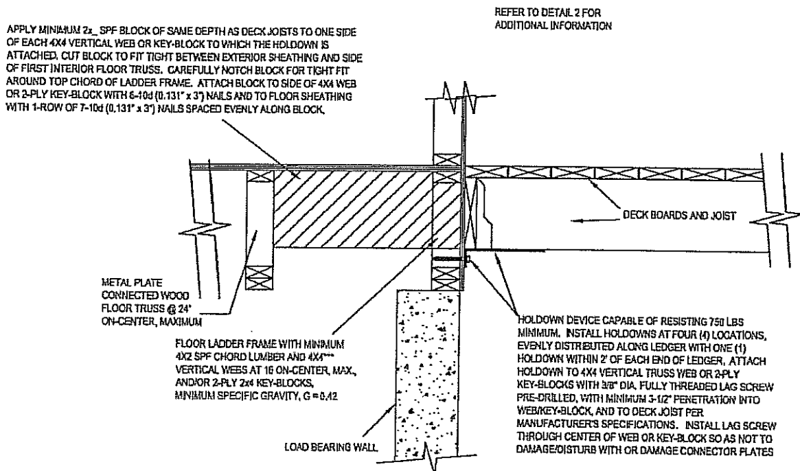
Detail 3: Deck Lateral Load Connection Capable of Resisting the 1500 lbf Lateral Load Requirement Specified in 2009 & 2012 IRC Section 507
