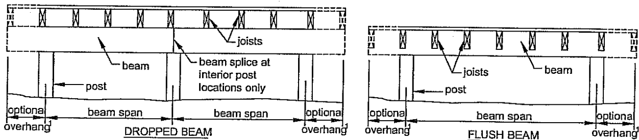
Figure 3 BEAM TYPES
