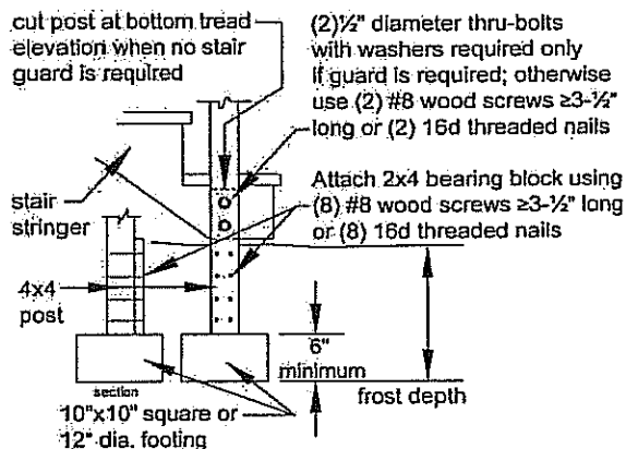
Figure 29 STRINGER BEARING
