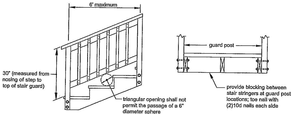
Figure 32 STAIR GUARDS
