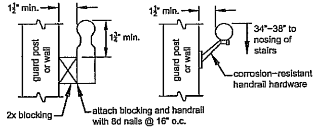
Figure 34 HANDRAIL GRASPABILITY
