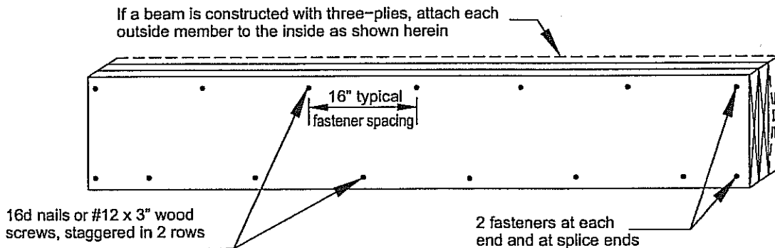
Figure 4 BEAM ASSEMBLY
