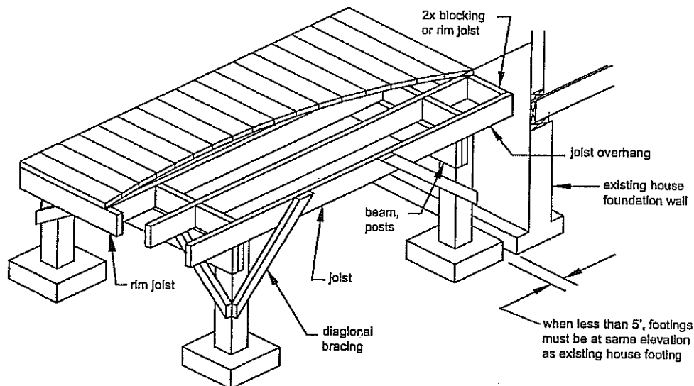
Figure 17 FREE-STANDING DECK
