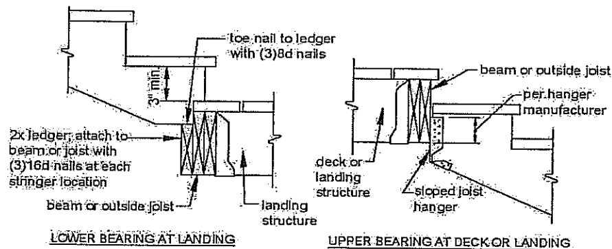
Figure 28 STRINGER BEARING
