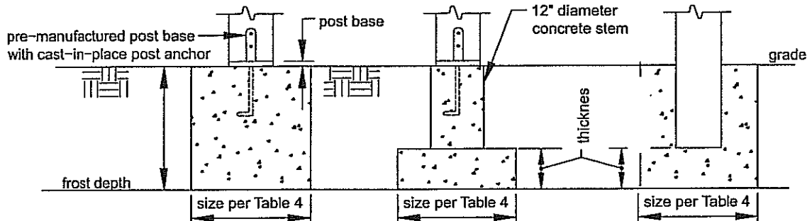
Figure 1 FOOTINGS
