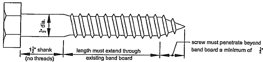
Figure 16 LAG SCREW
