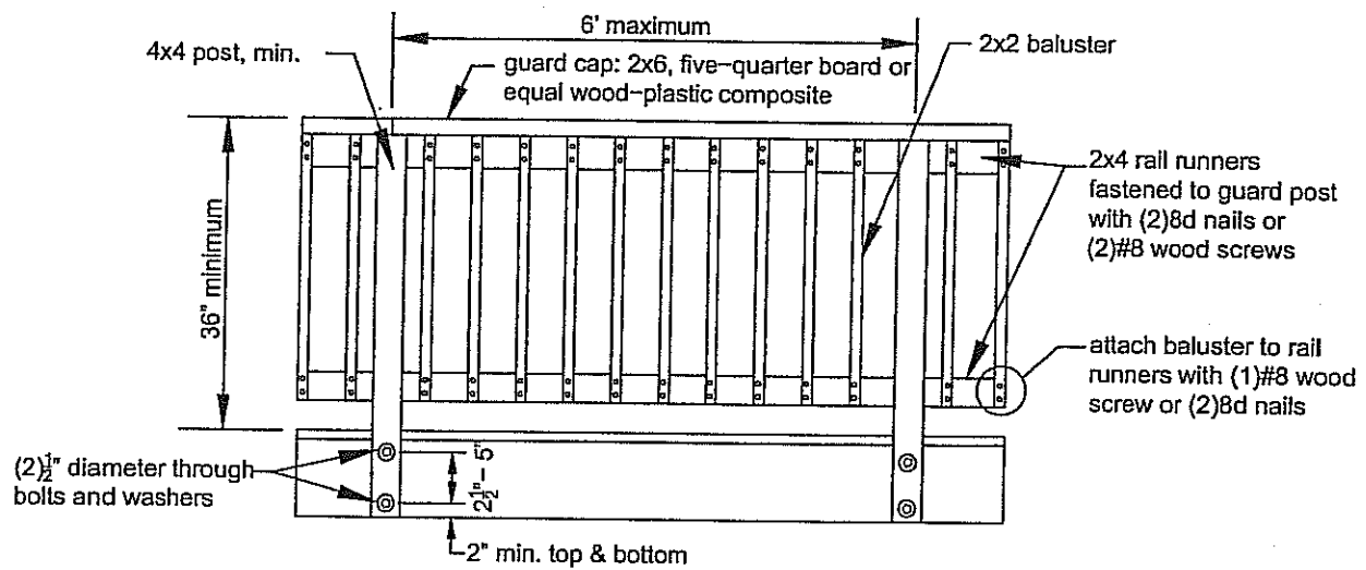
Figure 24 GUARDS
