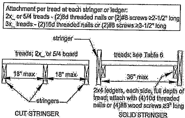
Figure 31 STAIRWAY TREADS
