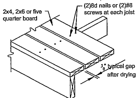
Figure 22 TYPICAL DECKING
