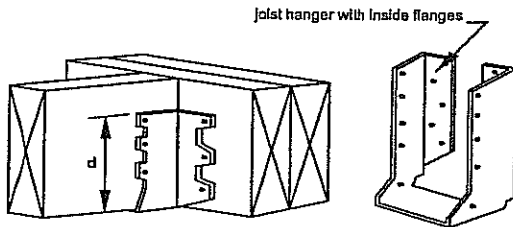
Figure 9 JOIST HANGERS
